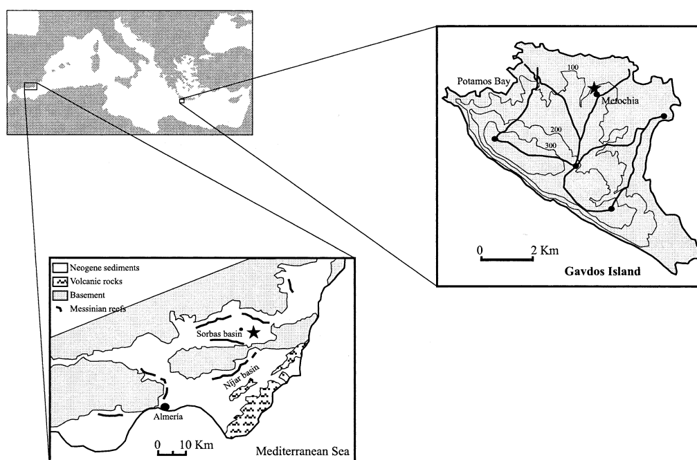
Fig. 1. Location maps of the Mediterranean Sea sections studied in this paper: west Mediterranean = southeast Spain; east Mediterranean = Gavdos Island (Greece). Sections are marked by stars.
