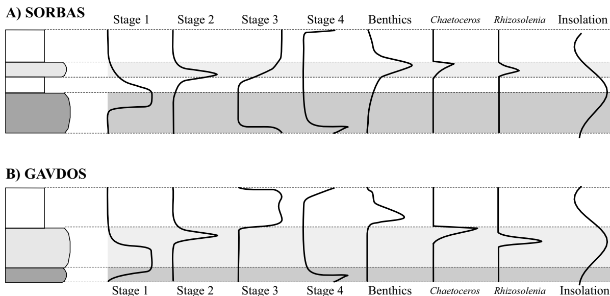
Fig. 8. Summary diagram showing similarities and differences between western (A) (Sorbas) and eastern (B) (Gavdos) Mediterranean Sea lithological and organic results during the Messinian. Dark gray: sapropel. Light gray: diatomite. White: homogeneous marl. Stage 1 represents warm-oligotrophic planktic foraminifera species; stage 2 represents Neogloboquadrinids and Globorotalia miotumida ; stage 3 represents Globigerina bulloides abundance, and stage 4 represents Globigerinita glutinata abundance. The abundance of benthic foraminifera, two diatom species, and a reference insolation cycle are also represented. All values increase to the right.
